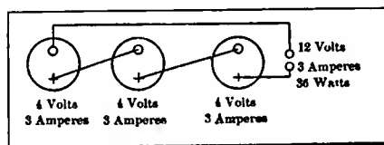
Fig. 3—Showing voltage and amperage when connecting batteries in series
